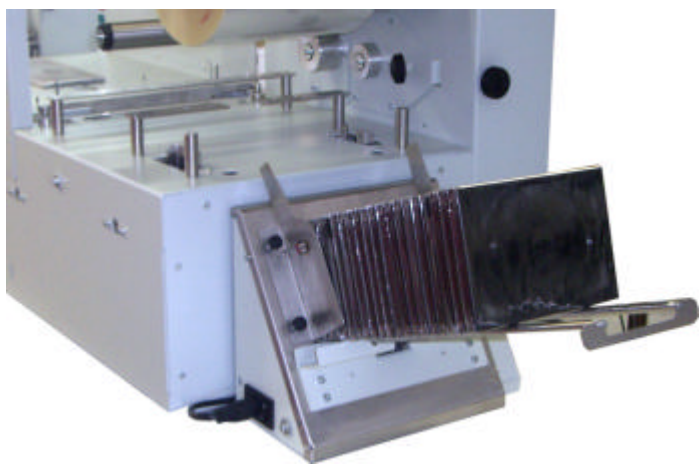
SpeedWrapper fitted with the Up-Stacker
